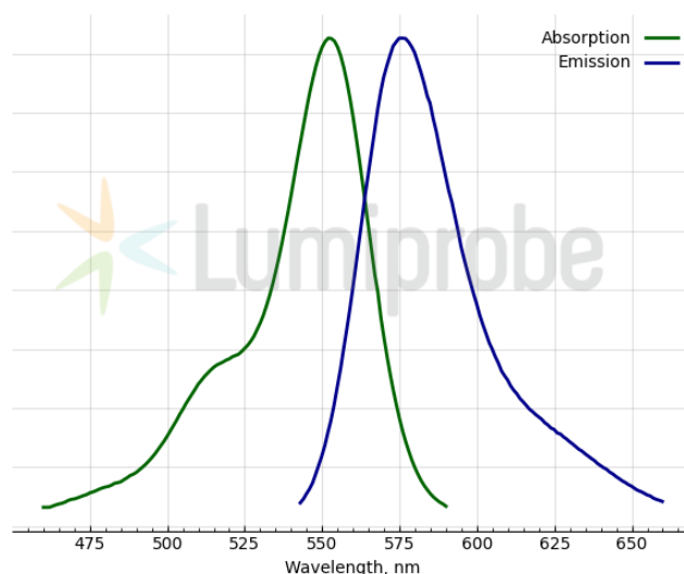
Excitation and emission spectra of TMRE
