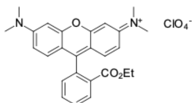
Structure of TMRE mitochondrial dye
