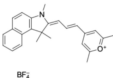
Structure of Pyrylium-6 (Py-6)
