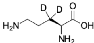
Structure of L-Ornithine-d2
