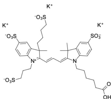
Structure of AF 555 carboxylic acid
